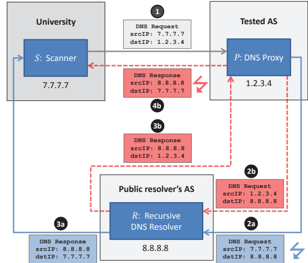
Figure 9: Network overview illustrating the two possible paths for DNS requests and responses for which the replying IP address did not match the IP address that was encoded in the requested domain
